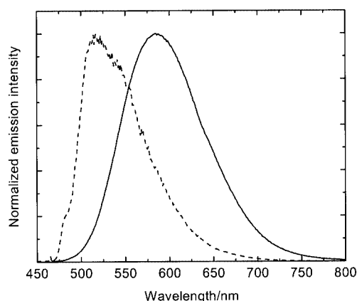
Figure 4. Emission spectra of complex 3 in \text{CH}_3\text{CN} at 298 K (---) and EtOH/MeOH (4:1, v/v) at 77 K (—)
