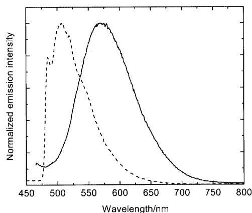
Figure 3. Emission spectra of complex 2 in \text{CH}_3\text{CN} at 298 K (---) and EtOH/MeOH (4:1, v/v) at 77 K (—)
