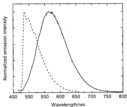
Figure 2. Emission spectra of complex 1 in \text{CH}_3\text{CN} at 298 K (---) and EtOH/MeOH (4:1, v/v) at 77 K (—)
