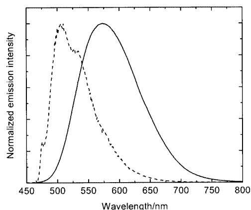
Figure 5. Emission spectra of complex 4 in CH 3 CN at 298 K (---) and EtOH/MeOH (4:1, v/v) at 77 K (-----)
