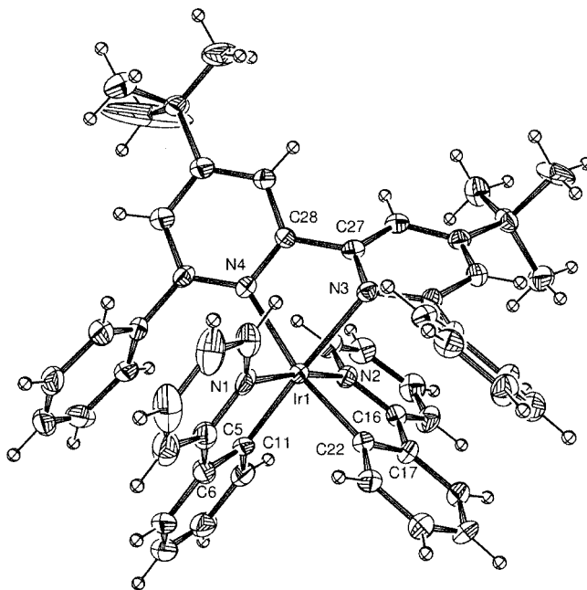
Figure 1. ORTEP representation of complex 1 ; the unit cell contains 1.5 molecules of H 2 O, which have been omitted for clarity, as has the PF 6 − counteranion
